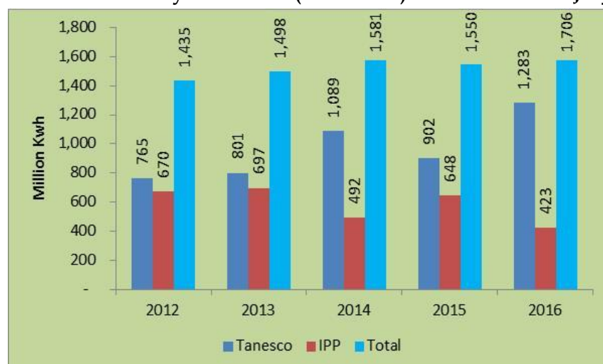
Chart 3: Electricity Generated (Mill. Kwh) for the Period of July - September, 2012 - 2016
