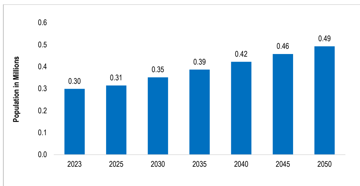
Figure 1.1: Projected Population Trends; Mbinga District Council, 2023 – 2050
