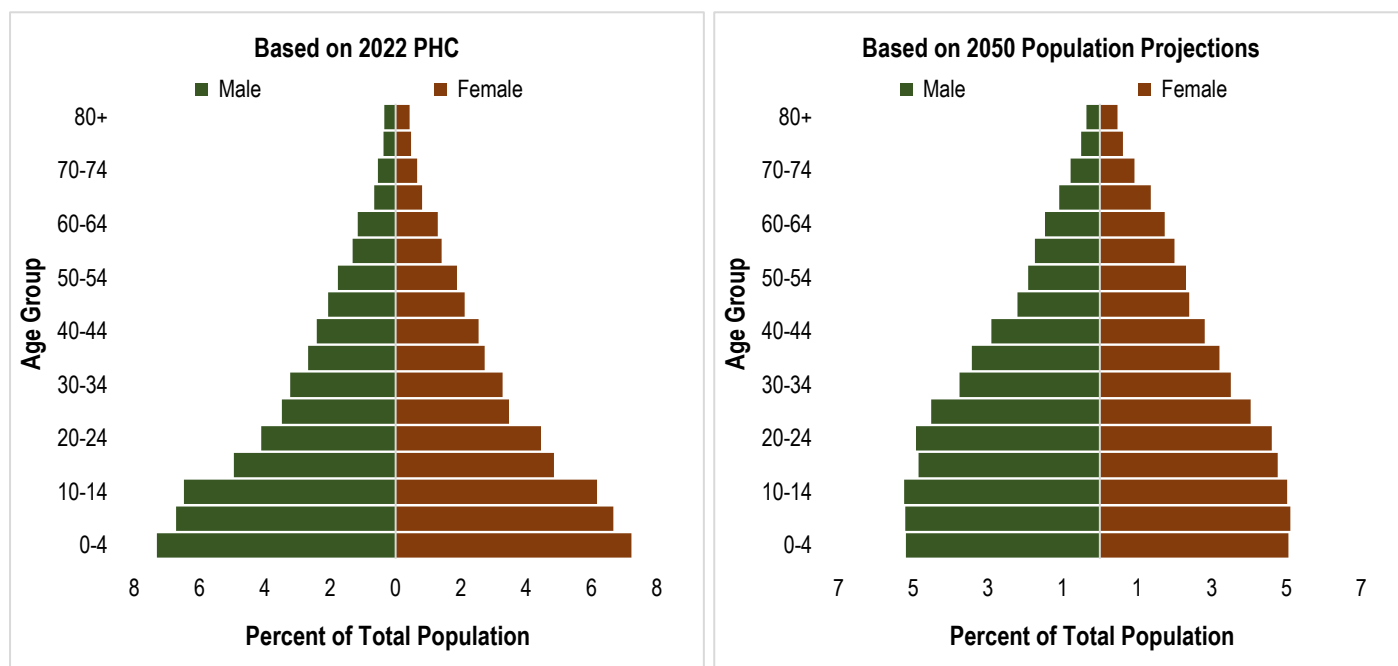
Figure 1. 4: Projected Population Pyramid for Five Year Age Groups; Mbinga District Council, 2022 and 2050
