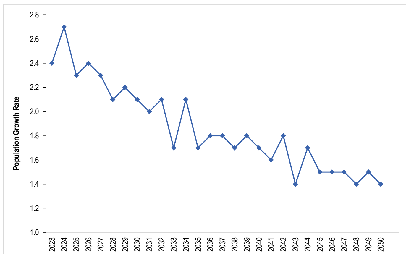
Figure 2. 1: Projected Population Growth Rates; Mbinga District Council, 2023 – 2050
