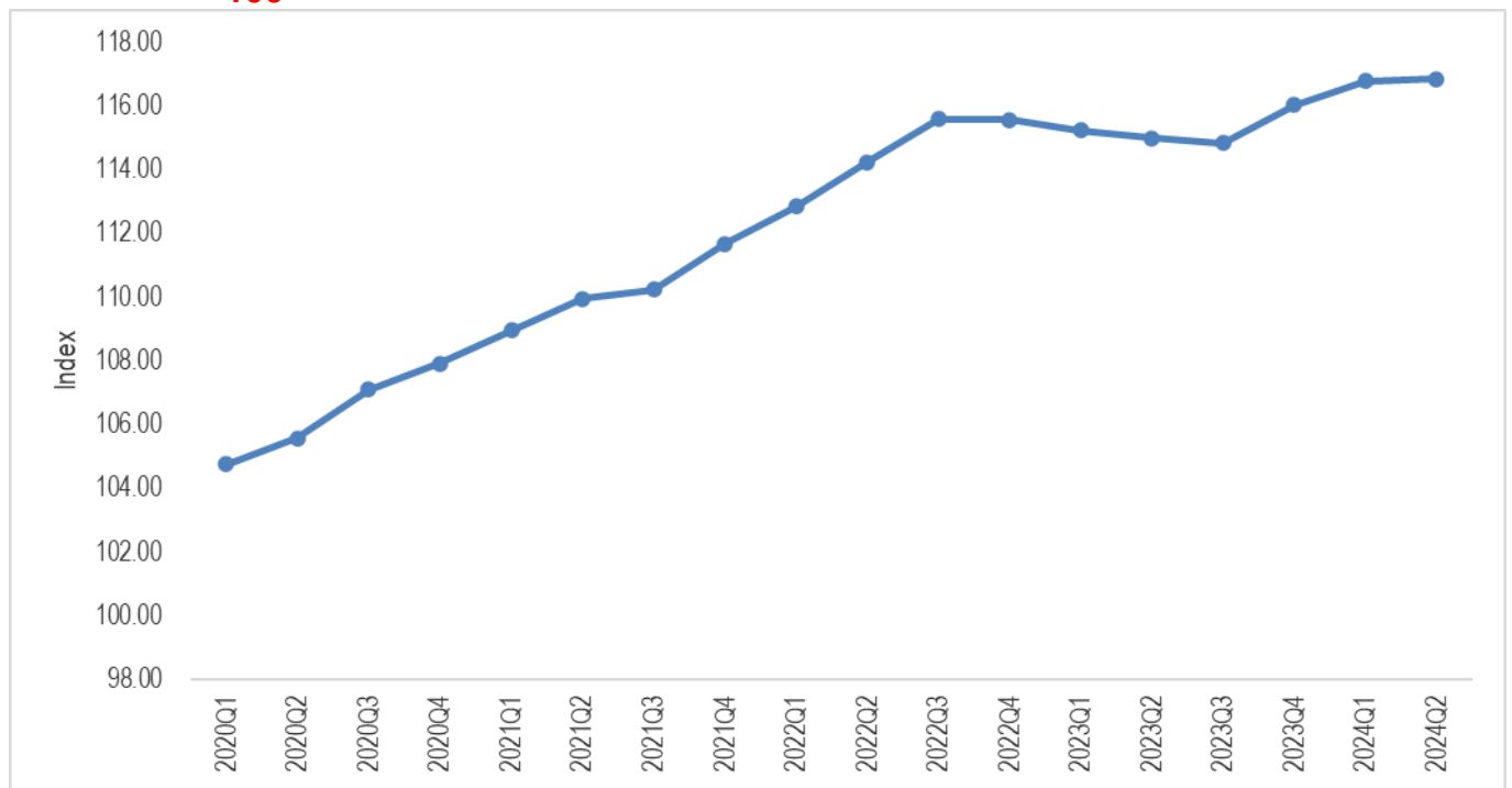
Chart 1: Overall Producer Price Indices for the Quarter Ending June 2024 (Dec 2018 = 100)
